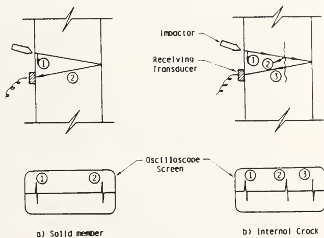
Fig. 2.5—Ultrasonic testing, pulse echo technique
